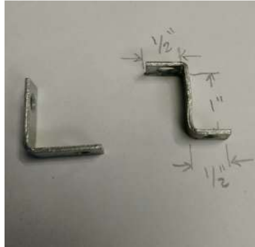
this is the dimensions to bend the plate (a 1-1/2" strap plate)
